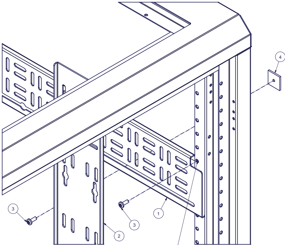
DETAIL A
