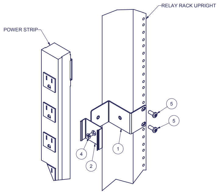
DETAIL A FOR TAPPED #12-24 UPRIGHT (M6 HARDWARE USED FOR M6 UPRIGHT)
